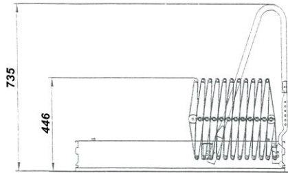
SIDE VIEW - CLOSED
