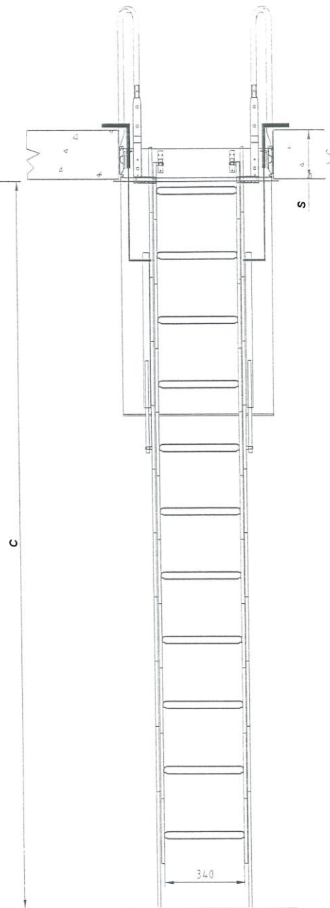
FRONT VIEW - OPEN
